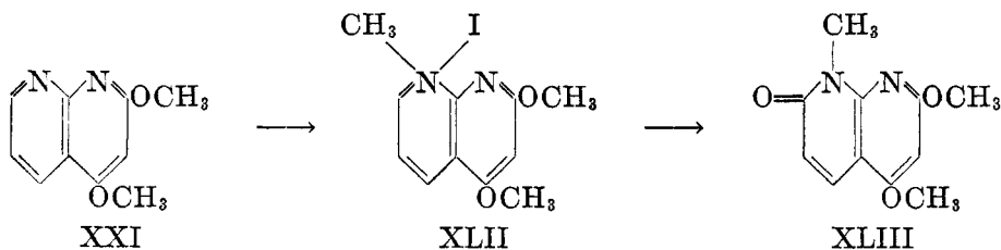
2,4-Dimethoxy-1,8-naphthyridine
