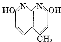
2,7-Dihydroxy-4-methyl-1,8-naphthyridine
